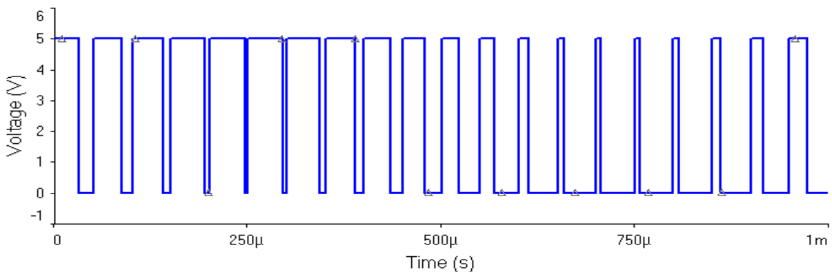
Fig 2.6 Graph of controlled square wave
