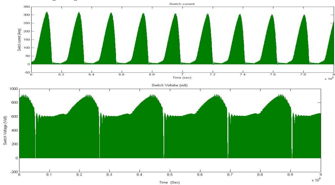
Fig 3.5 Switch Current And Voltage
