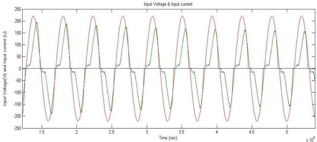
Fig 3.6 Input voltage and Current Waveform
