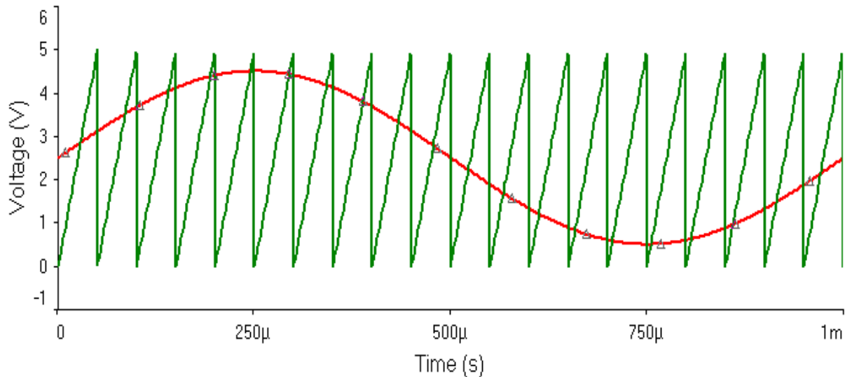
fig.2.5 Graph of Triangle wave and Sinusoidal control wave
