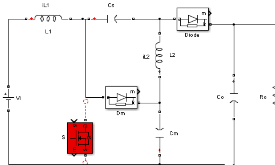
Fig.2.2 first operation stage
