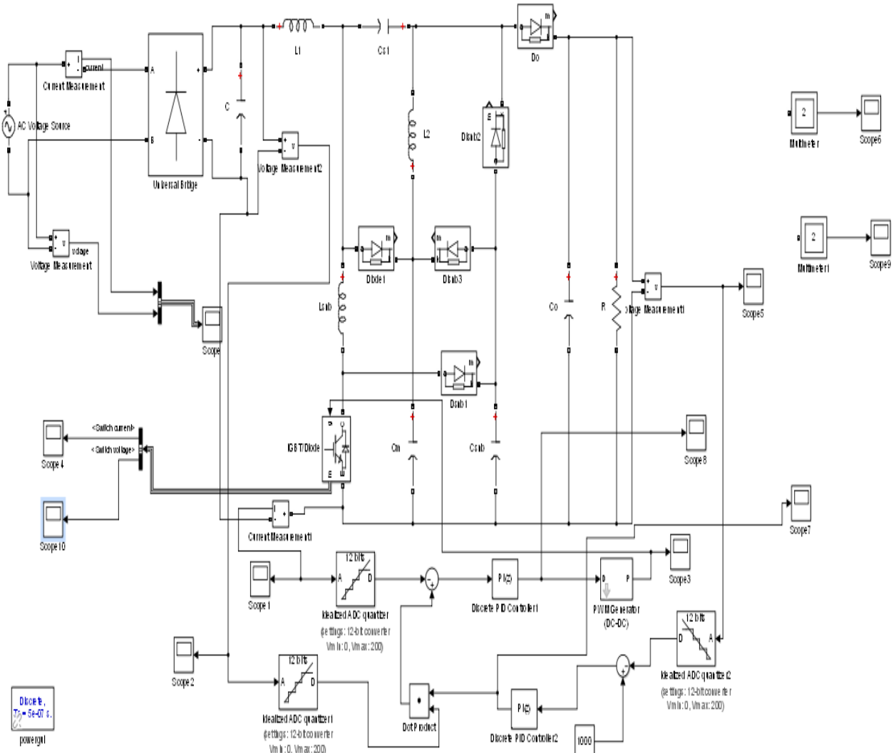
Fig 3.1 Simulation circuit of SEPIC converter
