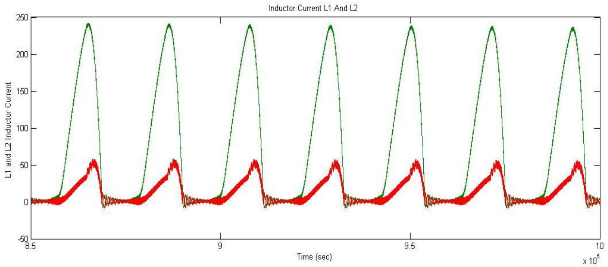
Fig.3.3 Inductor current L1 and L2 waveform
