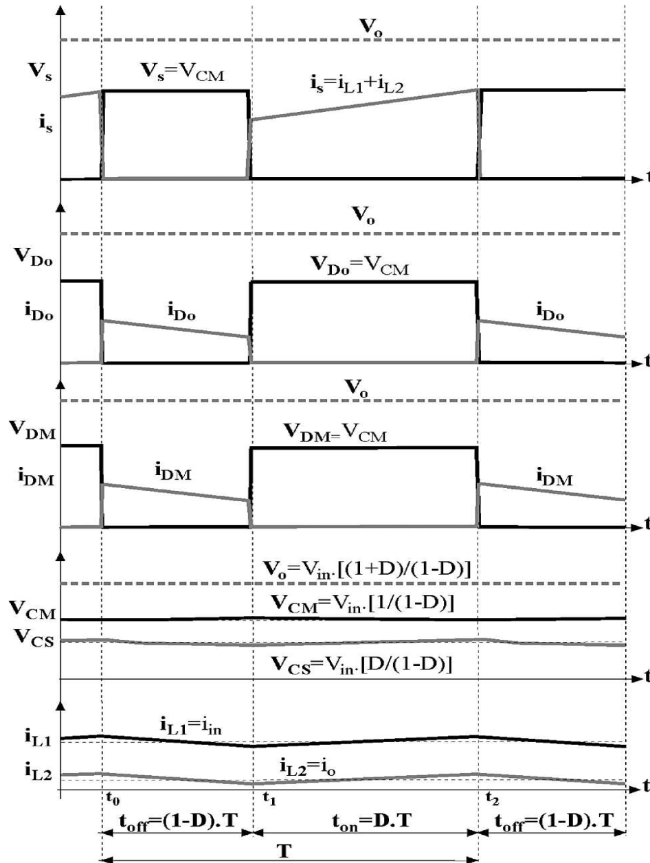
Fig.2.4 main theoretical waveforms operating with hard switching commutation
