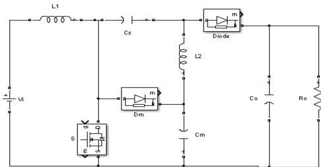
Fig 2.1 Modified SEPIC converter
